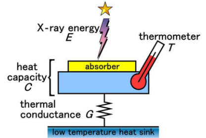
Fig. 6 Concept of X-ray micro-calorimeter
