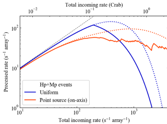
Fig. 9 Incoming vs. processed rate for Hp+Mp events (solid). Because of the limitation in the CPU load ("PSP limit"), the processed rate is reduced from what would otherwise be observed (dotted). The calculations do not include the effect by electrical crosstalk.
