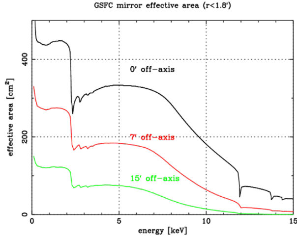
Fig. 4 Effective area (mirror only) as a function of energy at on-axis and some off-axis angles. The source extraction radius is 1.8 arcmin (78% encircled energy fraction). Note that this is a mirror-only effective area. Fig. 14 shows the actual effective areas combined with detectors.
