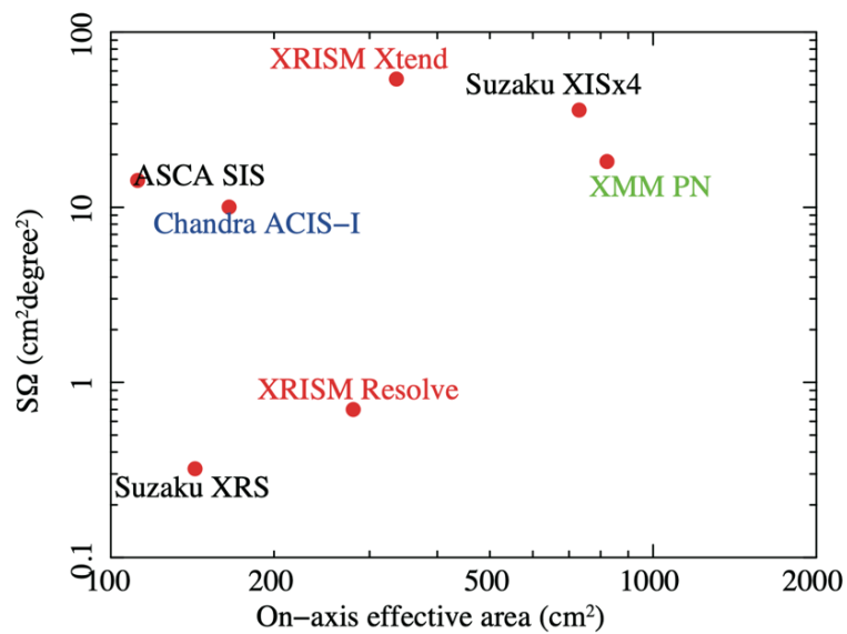
Fig. 19 Grasp vs on-axis effective area at 7 keV of Resolve and Xtend. Suzaku XIS, Chandra ACIS-I, XMM PN are also shown for comparison.
