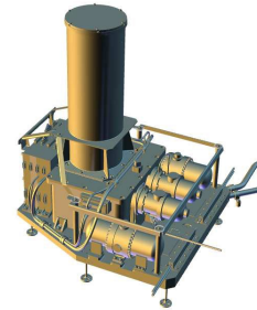
Fig. 11 External view of Hitomi/SXI [7]
