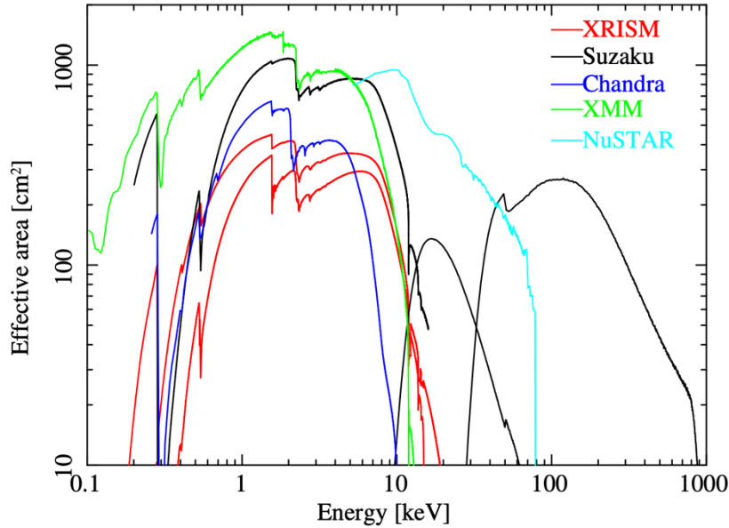
Fig. 16 On-axis effective area of XRISM (Resolve, Xtend), Suzaku (XIS-BI+XIS-2FI, HXD), Chandra (ACIS-S), XMM-Newton/EPIC (PN+MOS1+MOS2), and NuSTAR.
