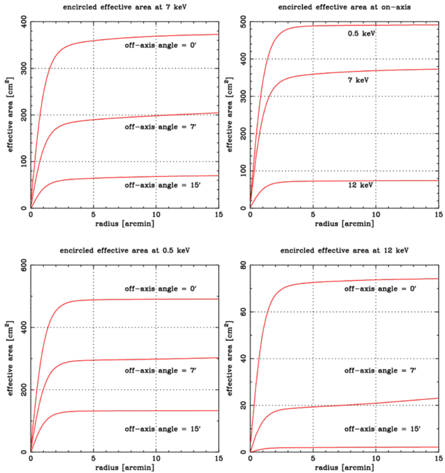
Fig. 5 Encircled effective area, representing the sharpness of an image at several energies at on-axis and some off-axis angles.
