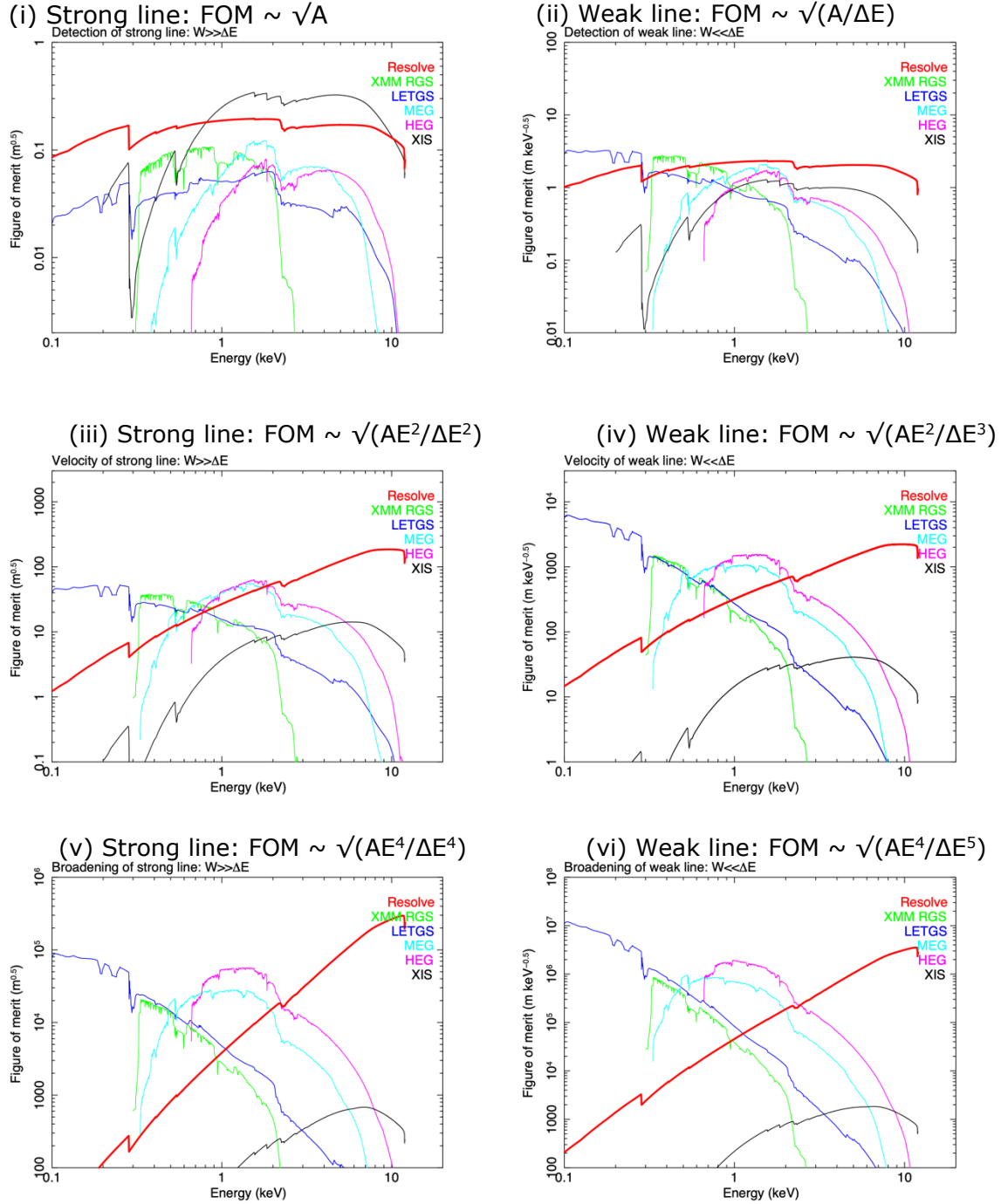
Fig. 17 Figures of merit (FOM) for (i) detection of strong line, (ii) detection of weak line, (iii) velocity of strong line, (iv) velocity of weak line, (v) broadening of strong line, (vi) broadening of weak line.
