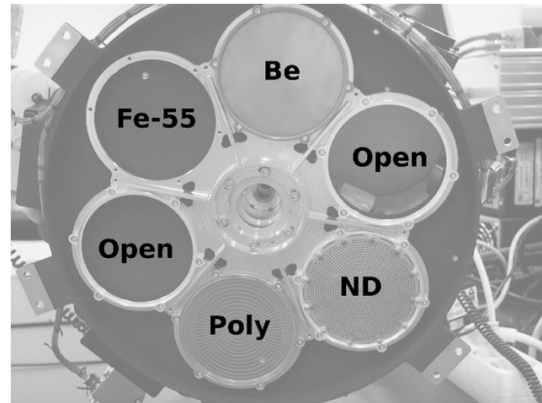
Fig. 10 Filter selection. The filter wheel has three filters, two open positions, and one position with a radioactive Fe-55 calibration source. The three filters are Beryllium filter (Be), neutral-density filter (ND), and polyimide filter (Poly).
