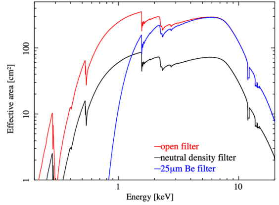
Fig. 15 Resolve on-axis effective area with filter: the open filter (red), neutral density filter (black), 25µm Be filter (blue).
