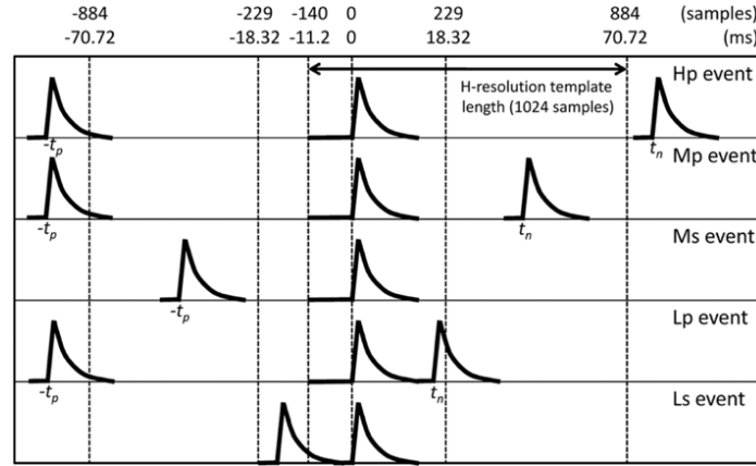
Fig. 8 Grade definition. The figure illustrates spacings of event pulses (shown with triangular shapes) corresponding to the five event grades: high-res (Hp) if there is no event triggered within \pm 70.72 ms; mid-res (Mp and Ms) if there is no event within \pm 18.32 ms; else low-res (Lp and Ls). "p"=primary denotes the earlier event of an event pair, while "s"=secondary denotes the later one. The minimum separations to distinguish the grades (70.72 ms for mid-res vs. high-res and 18.32 ms for low-res vs. mid-res) are determined primarily by the length of per-event pulse record that is required by the PSP to perform the signal processing called the optimal filter.
