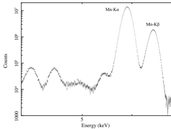
Fig. 12 ^{55}\text{Fe} Spectrum of a FM CCD chip in a ground calibration.
