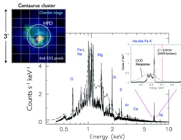
Fig. 7 Pixel layout (upper left panel). The array encompasses \sim 74% of photons of a point source at the center. Simulated spectrum of Centaurus cluster (bottom left).
