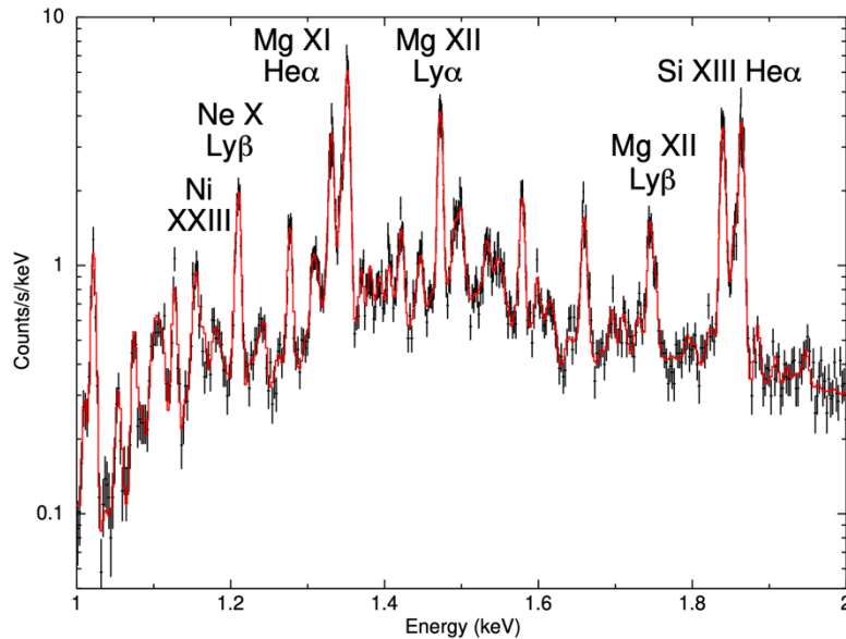
Fig. 22 100ks simulation of western half of 3C397. Several lines via Ni and Fe L-shell emission are seen for example at 1.045, 1.156 keV for Ni and 1.01 keV for Fe, respectively as well as peaks from K-shell transition of Si (1.84 keV) and Mg (1.33 keV).
