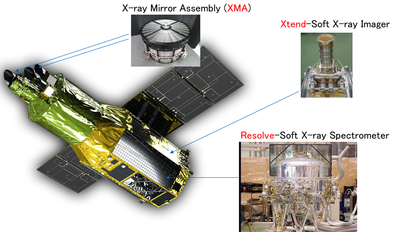
Fig. 2 Schematic view of the XRISM satellite. There are two focusing X-ray telescopes mounted at a fixed optical bench. They will focus X-rays onto focal plane detectors mounted on the base plate of the spacecraft.
