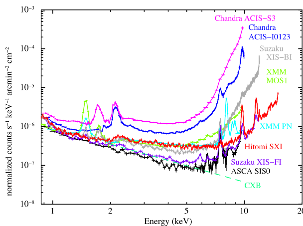
Fig. 13 Comparison of the sky background of X-ray CCD cameras [8]
