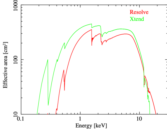
Fig. 14 On-axis effective area of XRISM telescopes & detectors, Resolve (red) and Xtend (green). For Xtend, the in-orbit performance of Hitomi/SXT+SXI is plotted here.
