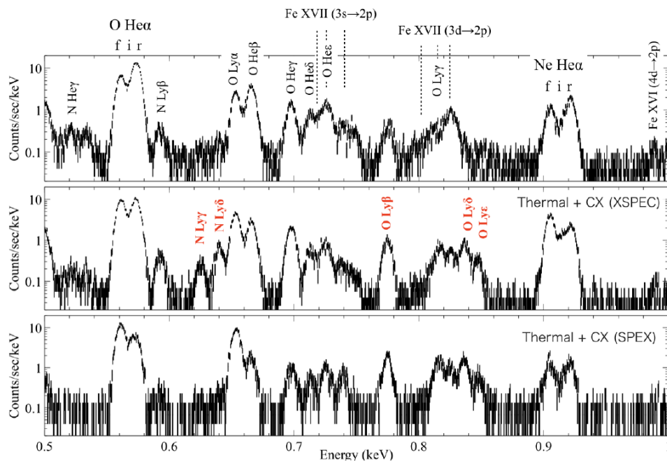
Fig. 23 30-ks simulated Resolve spectra of a shell region of the Cygnus Loop. Top: Assumed model is a typical thermal plasma with electron temperature of 0.2 keV. Middle: Same as the top panel but added a charge-exchange model in XSPEC. Bottom: Same as the middle panel but simulated in SPEX with similar model parameters.
