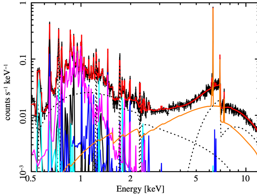
Fig. 21 A simulated spectrum of the obscured AGN Mrk 3 with a 200 ks Resolve observation. The model is based on a prior Suzaku observation.
