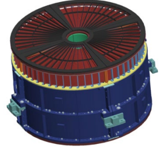
Fig. 3 Schematic view of XMA. The blue and red parts are the mirror housing and Pre-Collimator, respectively.
